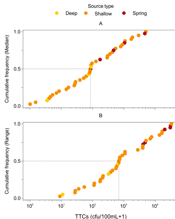
Fig. 2. Empirical cumulative distribution functions of (A) median TTCs and (B) range in TTCs for each water sources ( n > = 40 ).
